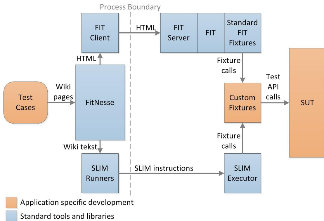
Figure 13: FitNesse's architecture [64]
